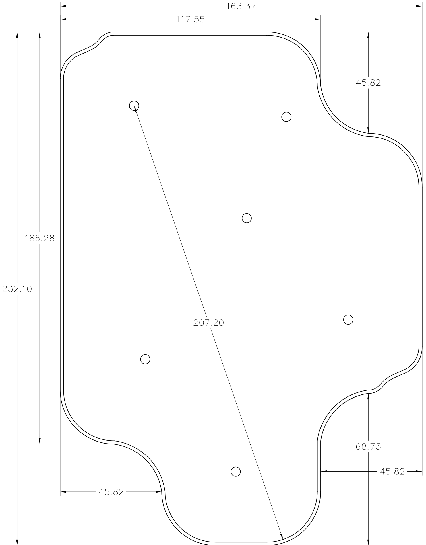
Professional 14x20 Putting Green (NTPG-59PP-1) (All Dimensions Shown Are Approximate)
